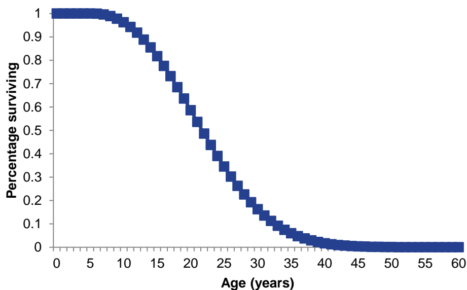
Figure 8. Freezers—Survival Function 486
