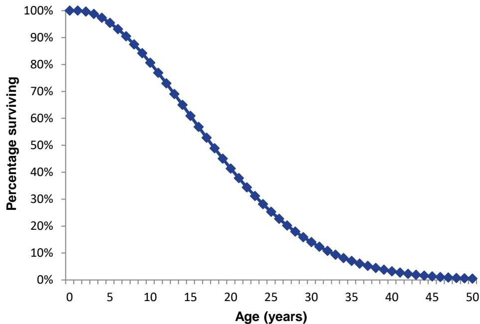
Figure 1. Central and Mini-Split AC/HPs—Survival Function 112
