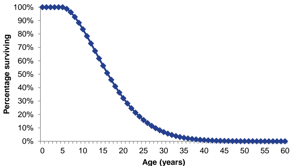
Figure 7. Refrigerators—Survival Function 467
